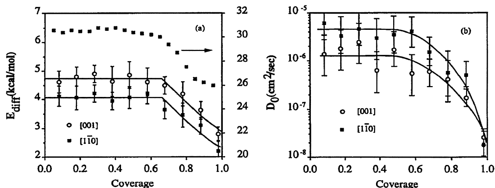
Fig. 16. Coverage dependance of anisotropic CO diffusion on Ni(1 1 0) obtained from LOD observations: (a) diffusion barriers along with the coverage dependence of the desorption energy; (b) corresponding prefactors. From [287].
