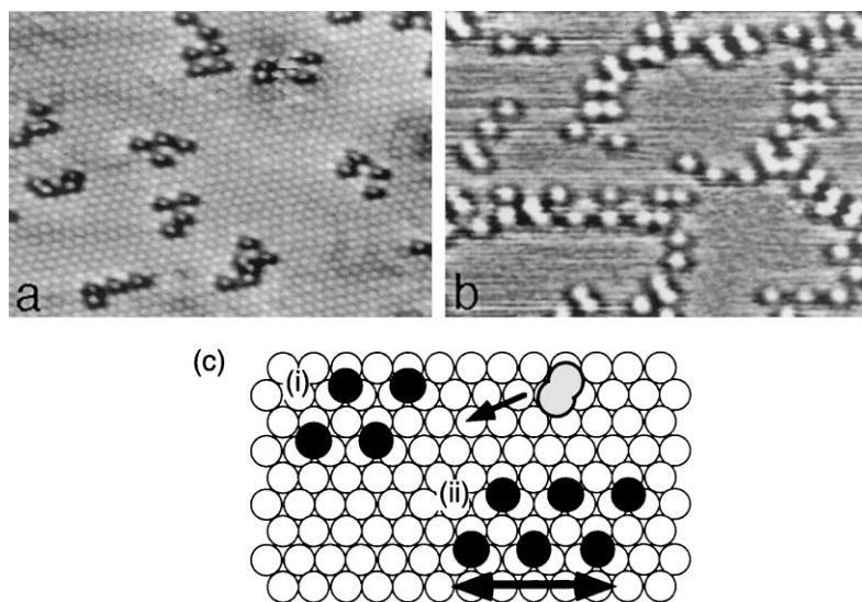
Fig. 36. Precursor-mediated aggregation of atomic oxygen in low-temperature adsorption of \text{O}_2 on \text{Pt}(1\ 1\ 1) . (a) At T = 140\ \text{K} groups consisting of 4–6 \text{O}_{\text{ad}} -atoms have formed from dissociation of 2–3 molecules (3 L dose, image 100 \times 60\ \text{\AA}^2 with the Pt atomic lattice resolved). (b) The one-dimensional islands from strings of O-pairs in [1\ \bar{1}\ 0] at T = 105\ \text{K} reflect an increased precursor lifetime at the surface and anisotropic precursor–atom interactions (1 L dose, image 70 \times 40\ \text{\AA}^2 ). (c) Schematic illustration of the one-dimensional growth of \text{O}_{\text{ad}} -chains. In (i) an oxygen precursor molecule (shaded) approaches an atom island; (ii) on its dissociation a chain string evolves. From [528].
