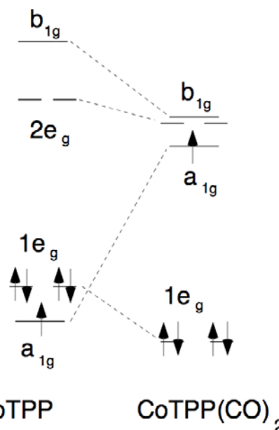
Fig. S2: Selected orbital energy levels for gas-phase CoTPP (left) and CoTPP(CO) 2 (right) taken from Ref. 1. The a 1g level has a large contribution from the Co d z 2 atomic level and is singly occupied. The 1e g orbitals correspond to d xz and d yz Co orbitals. The 2e g orbitals are the LUMO of CoTPP and are \pi -orbitals of the ligands. The b 1g orbital has a large contribution from the Co d x 2 -y 2 orbital. When two apical CO's are adsorbed the a 1g level is promoted and the b 1g reduces its energy 1 .
